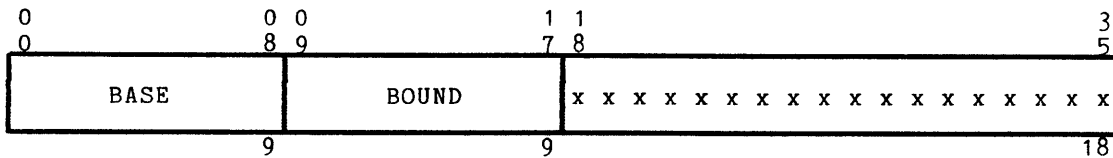
Figure 3-8. Base Address Register (BAR) Format
