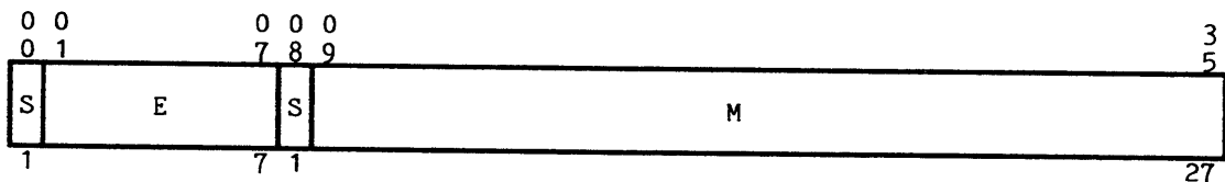
Figure 2-8. Single-Precision Floating-Point Binary Operand Format
