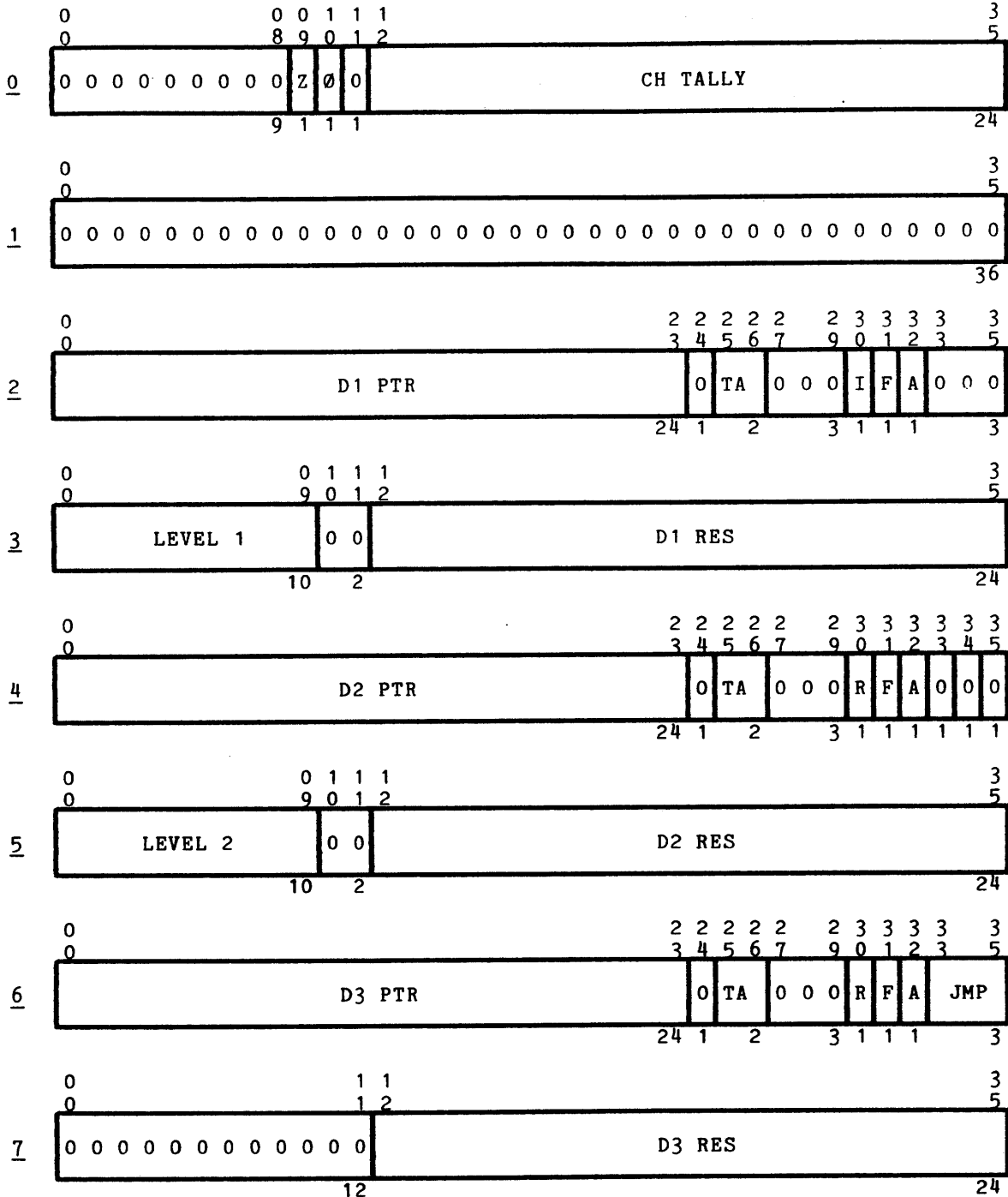
Figure 3-33. Decimal Unit Data Format
