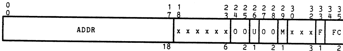
Figure 5-6. Page Table Word (PTW) Format
