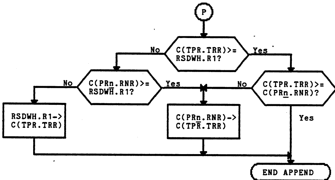
Figure 8-1(cont). Complete Appending Unit Operation Flowchart
