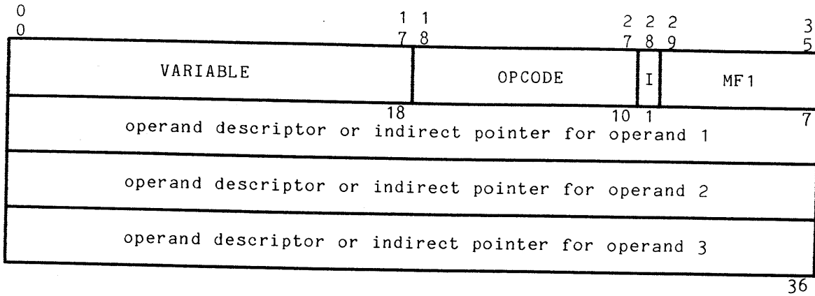
Figure 4-3. EIS Multiword Instruction Format
