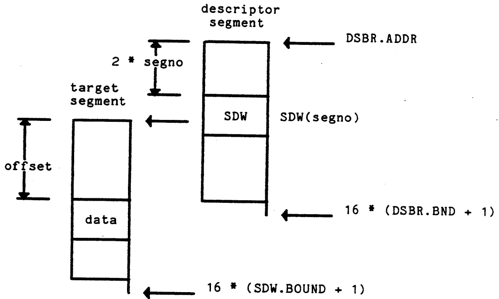
Figure 5-1. Main Memory Address Generation for Unpagged Segments
