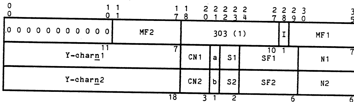
Figure 4-20. Compare Numeric (cmpn) EIS Multiword Instruction Format
