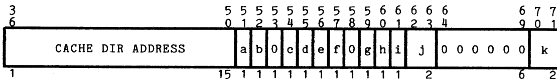
Figure 3-22. Cache Mode Register (CMR) Format - DPS and L68
