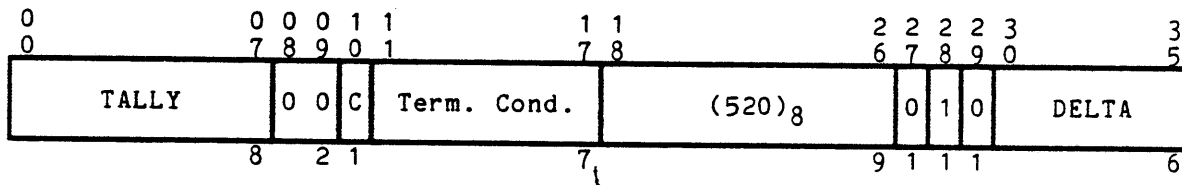
Figure 4-11. Repeat (rpt) Instruction Word Format
