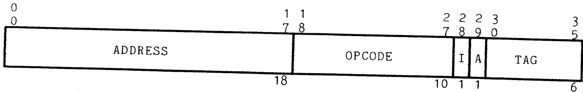
Figure 4-1. Basic and EIS Single-Word Instruction Format
