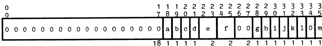
Figure 3-21. Mode Register (MR) Format - DPS 8M
