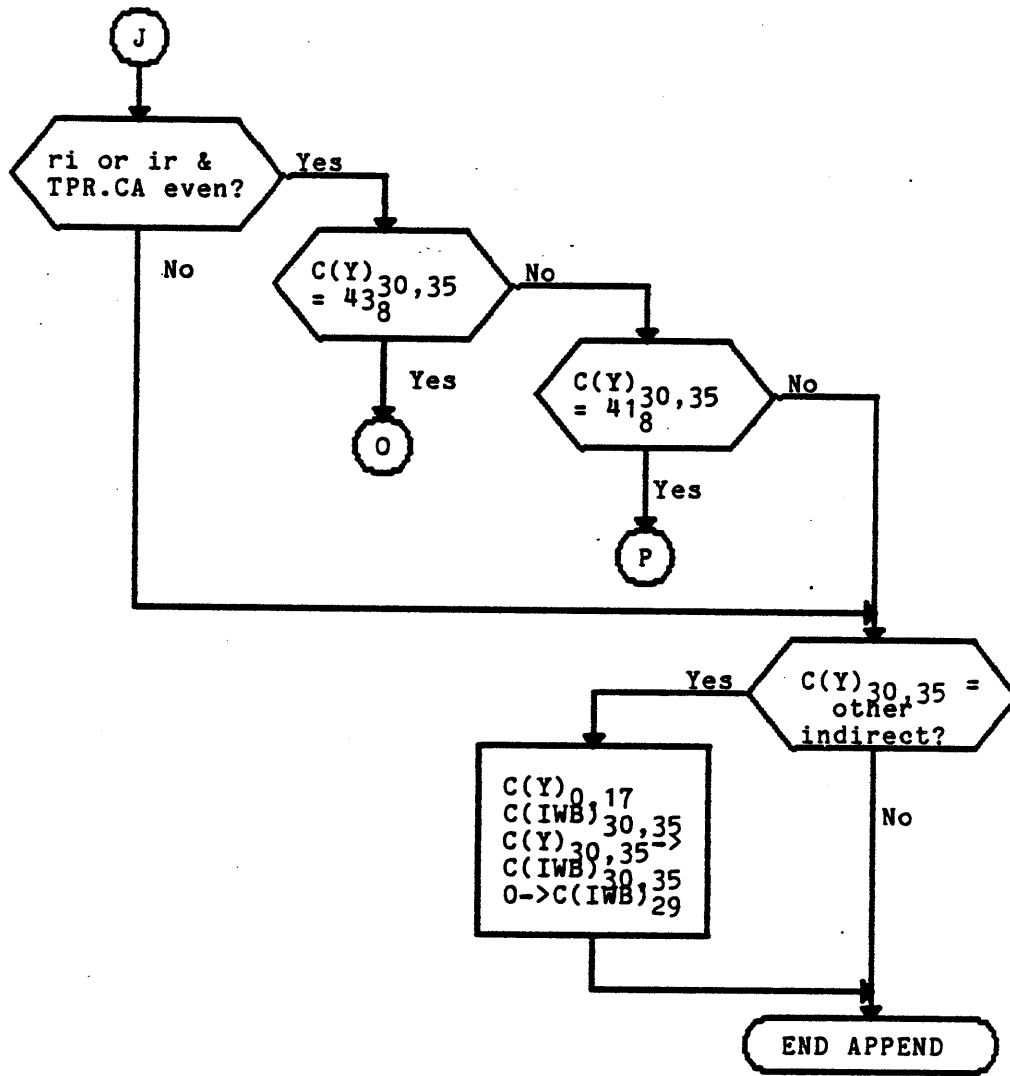
Figure 8-1(cont). Complete Appending Unit Operation Flowchart
