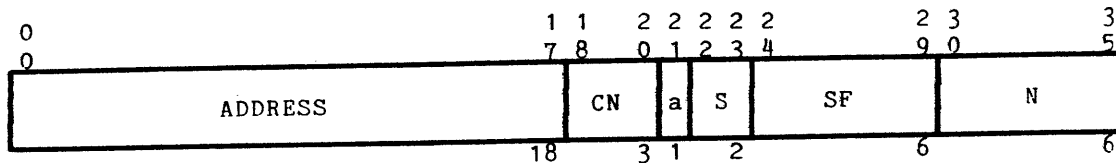
Figure 4-7. Numeric Operand Descriptor Format
