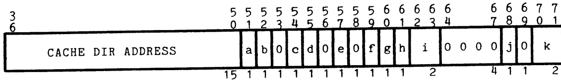
Figure 3-23. Cache Mode Register (CMR) Format - DPS 8M
