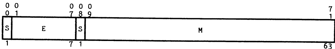
Figure 2-9. Double-Precision Floating-Point Binary Operand Format
