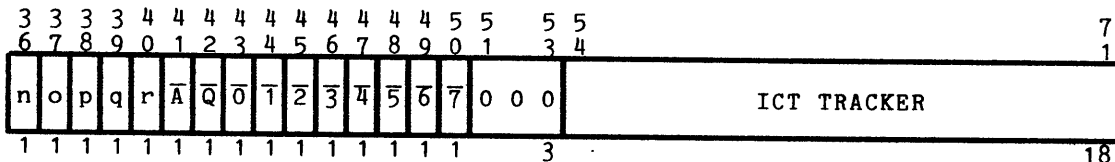
Figure 3-26. Operations Unit (OU) History Register Format
