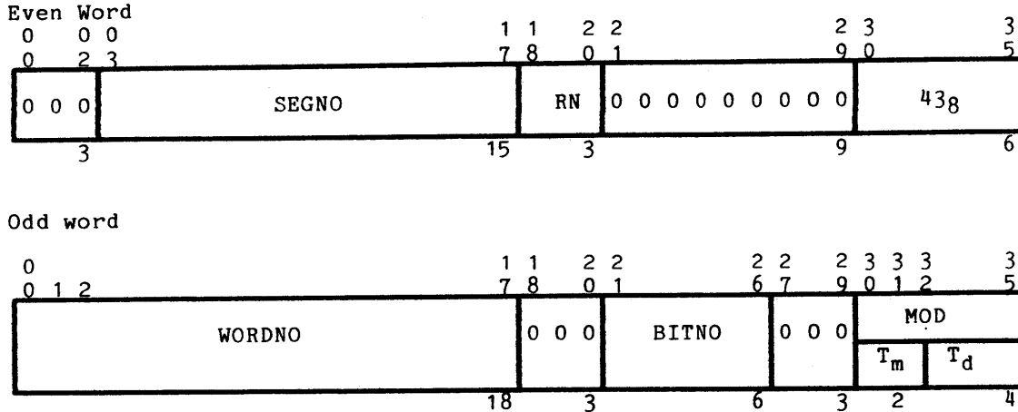
Figure 6-9. ITS Pointer Pair Format
